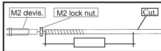
Elevator pushrod.
