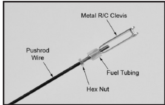
Elevator pushrod.
