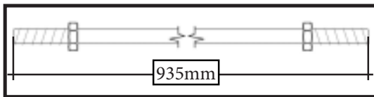
Rudder pushrod.
